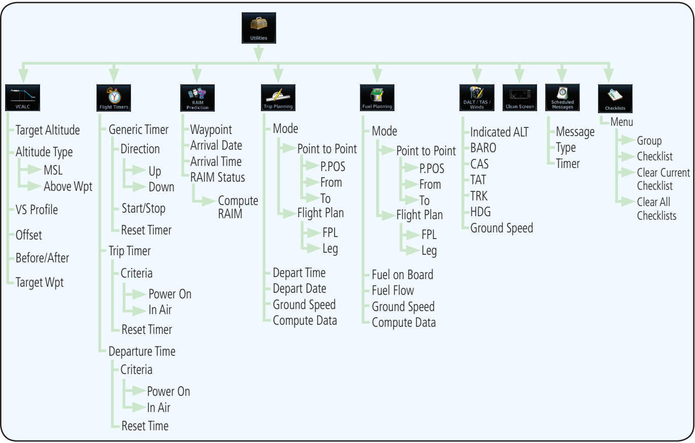
Figure 14-2 Utilities Functional Diagram
