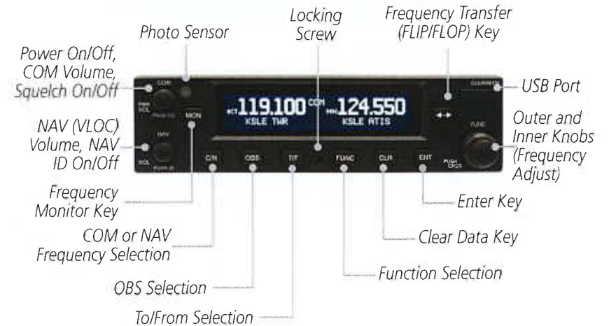
GNC 255 Front Panel Description
